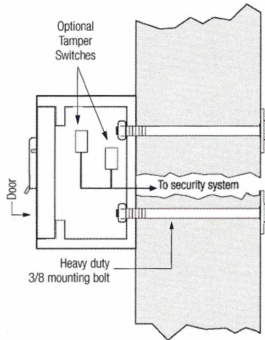
5000 Surface Mount with tamper switch
