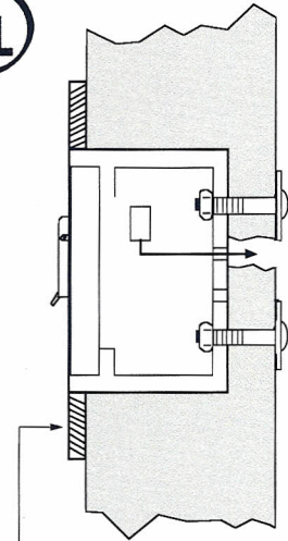
5000R Recessed Mount with flange
